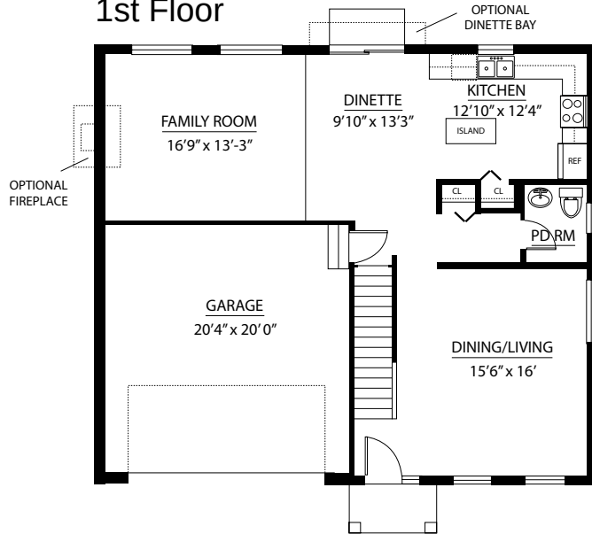
1st Floor
